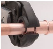
2. Align the jaws
