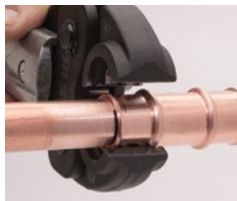
1. Insert the tube
