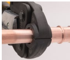
3. Pull the trigger
